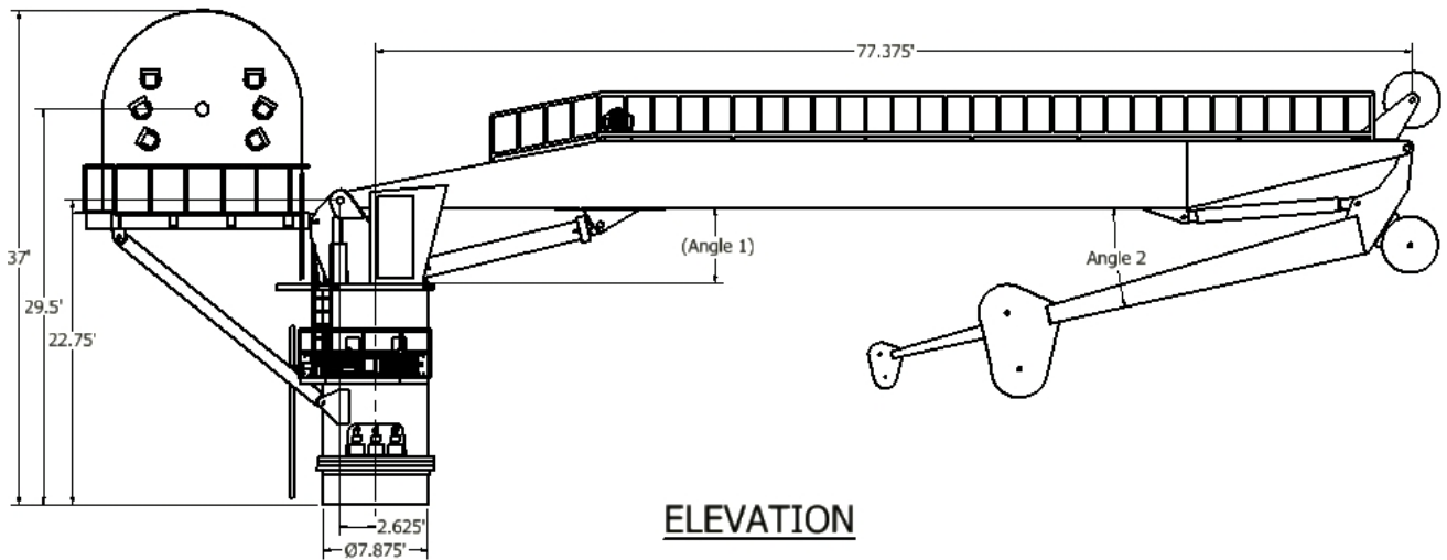
K-200 SIDE VIEW
